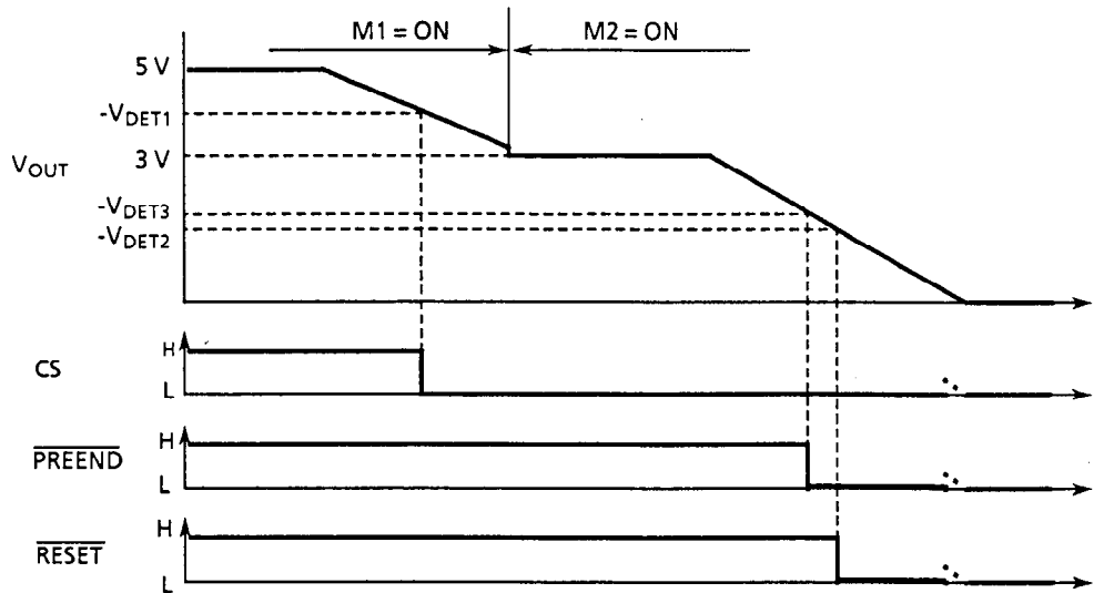
Figure 11 Detection potentials of voltage detectors
